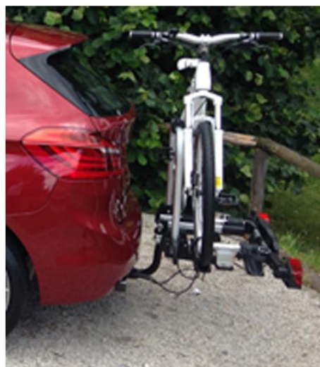
Compact rear bicycle carrier
